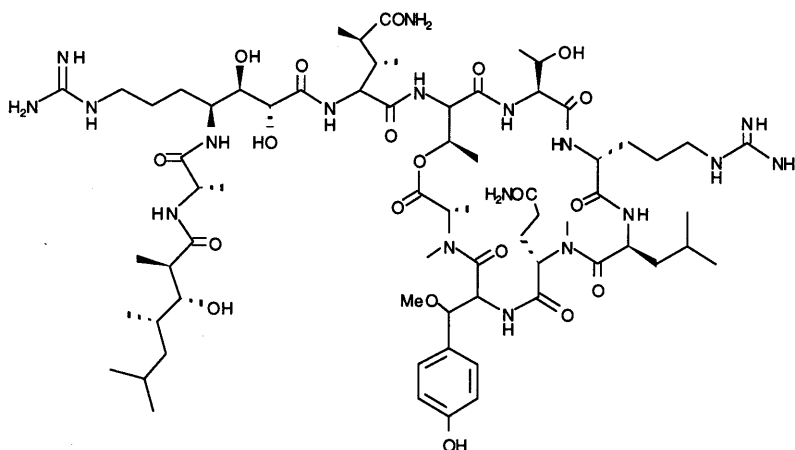
1 Callipeltin A
